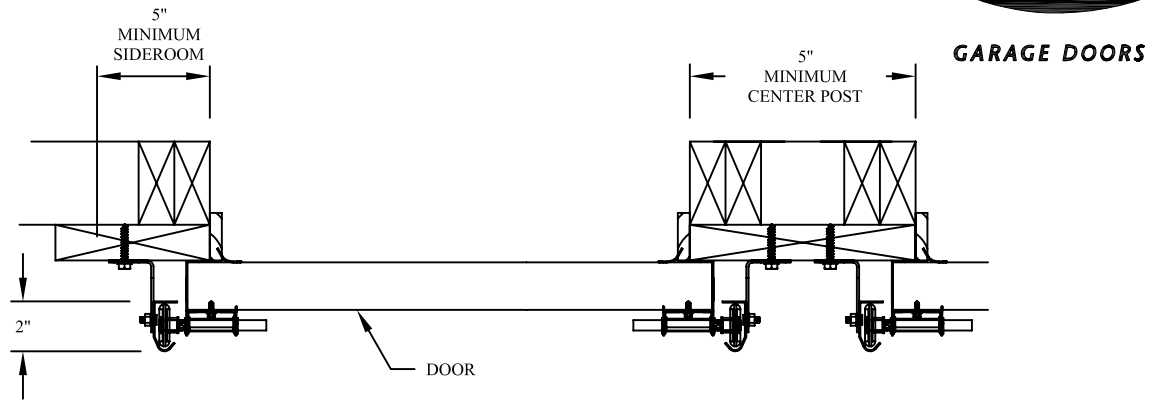
COMMERCIAL BRACKET MOUNT TO WOOD JAMB DETAIL
